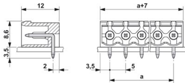
Dimensioned drawing
