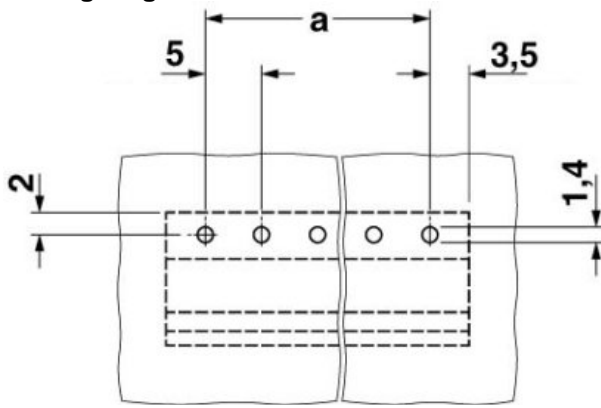
Dimensioned drawing
